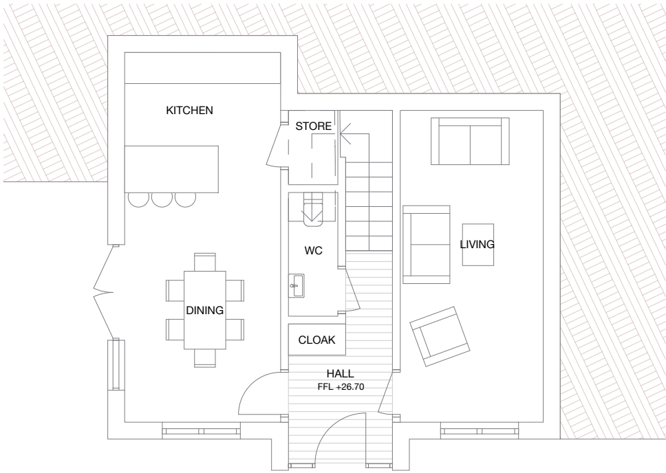
PROPOSED GROUND FLOOR PLAN SCALE 1:100 [A1]
