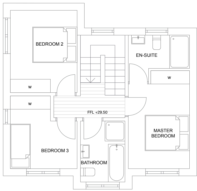
PROPOSED FIRST FLOOR PLAN SCALE 1:100 [A1]
