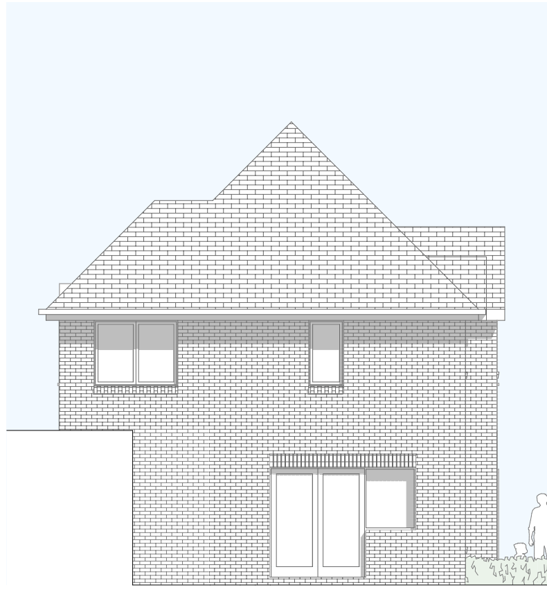
PROPOSED SIDE ELEVATION (SOUTH) SCALE 1:100 [A1]
