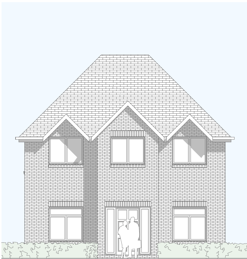
PROPOSED FRONT ELEVATION (EAST) SCALE 1:100 [A1]
