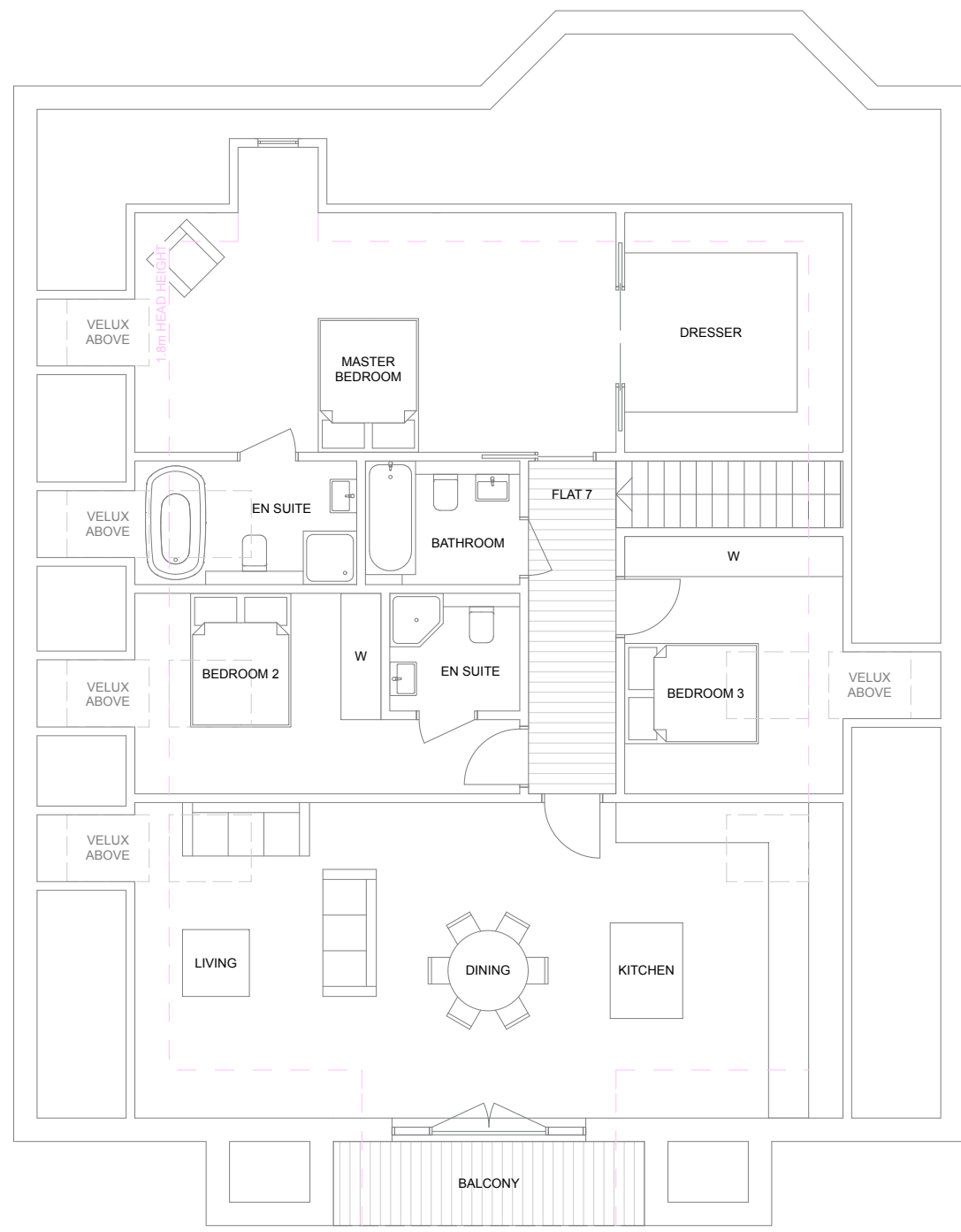
PROPOSED SECOND FLOOR PLAN SCALE : 1:100 [A1]
