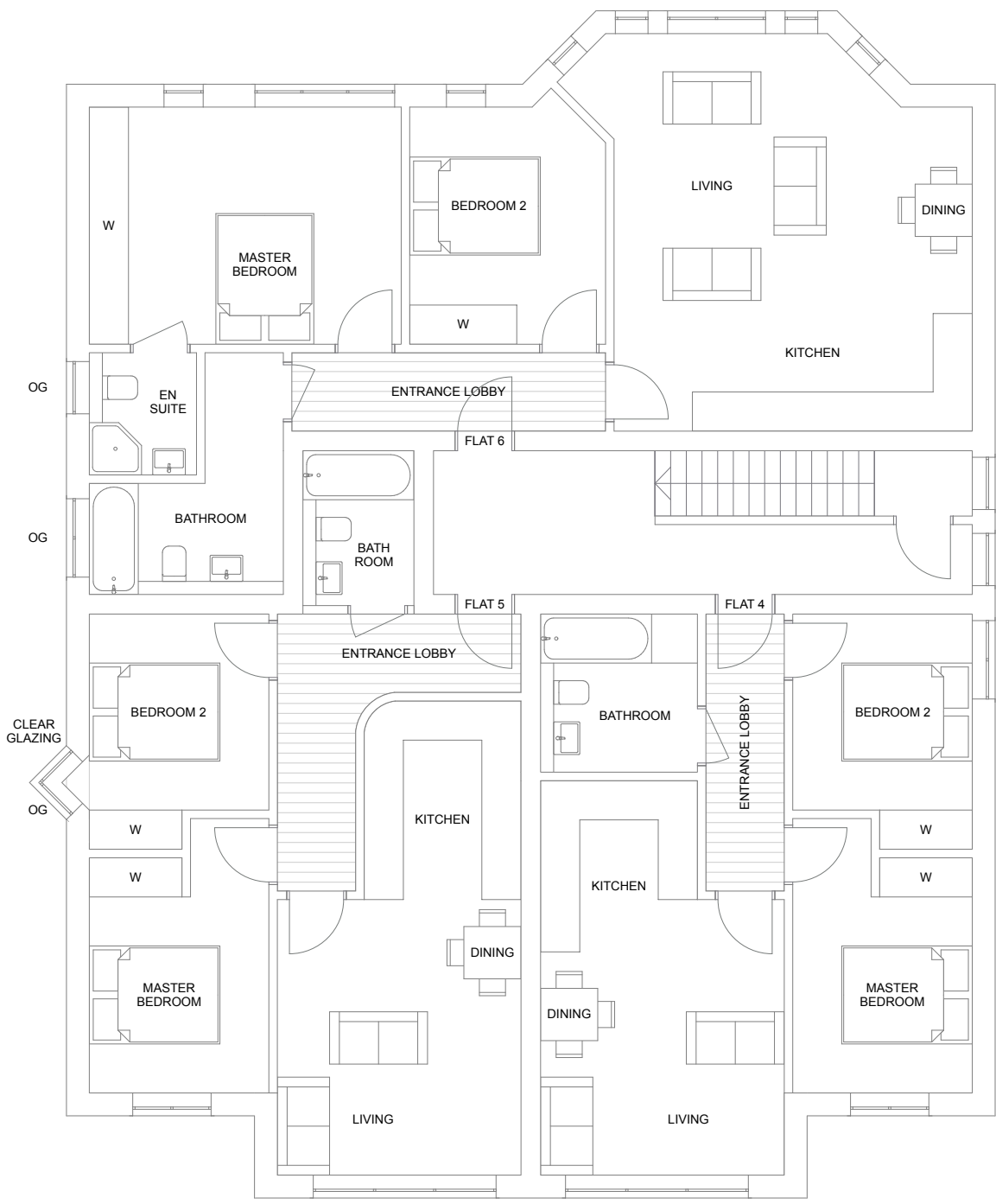
PROPOSED FIRST FLOOR PLAN SCALE : 1:100 [A1]
